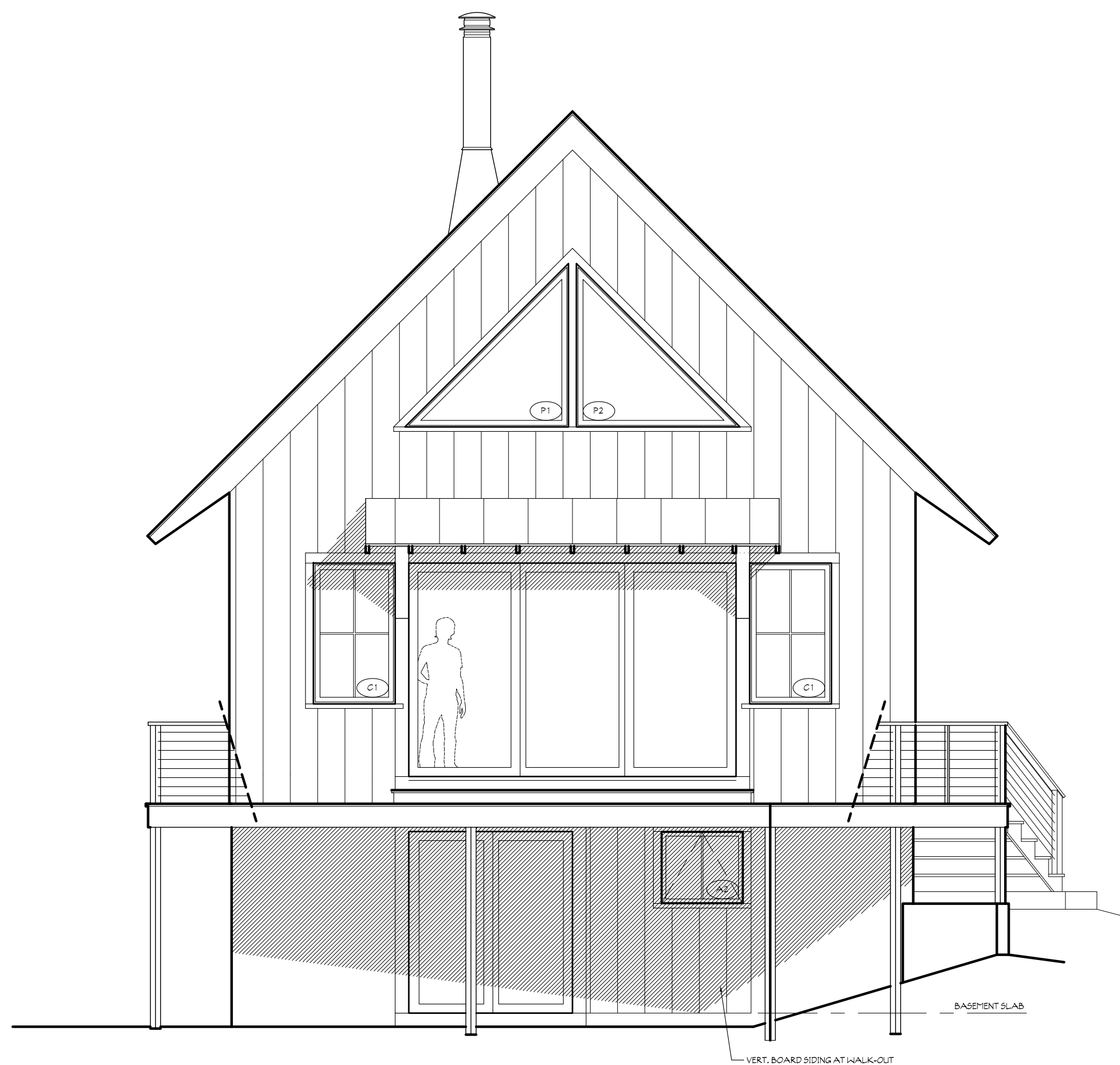
NORTH ELEVATION 1/4" = 1'-0"
