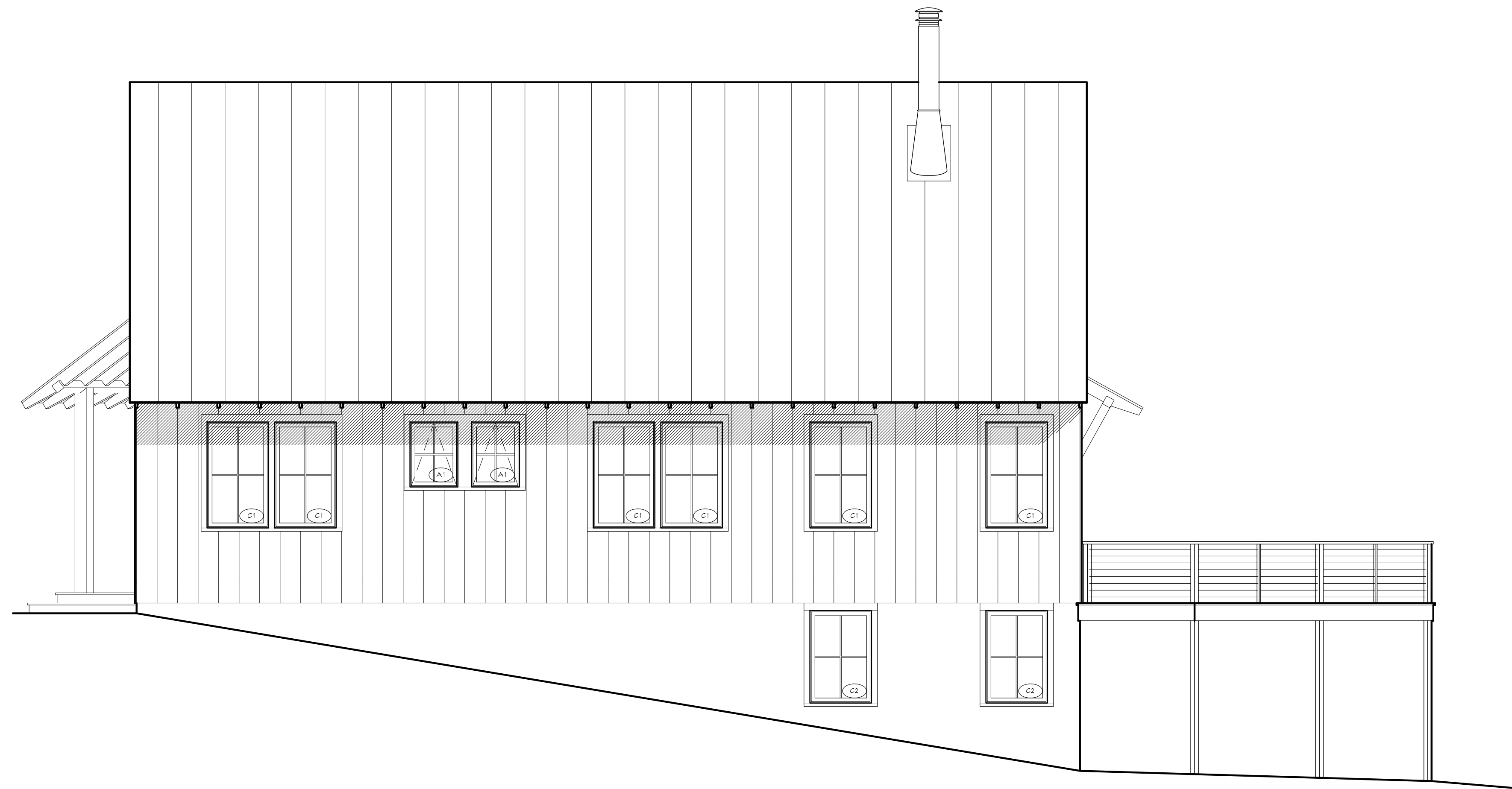
EAST ELEVATION 1/4" = 1'-0"
